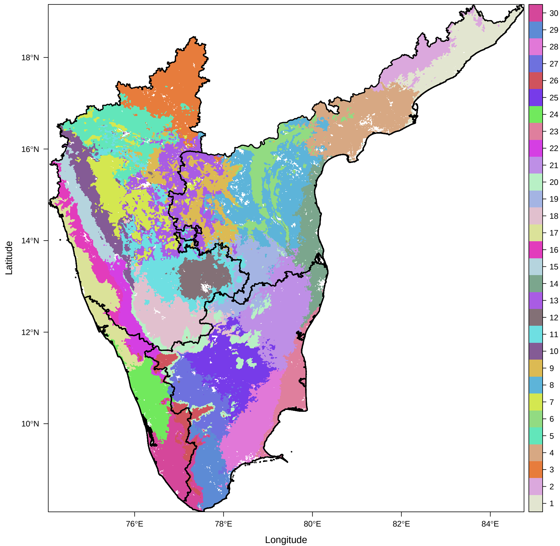
present seed zones south_India – 30 clusters
